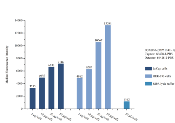
Sample test of MP51341-1, FOXO3A Monoclonal Matched Antibody Pair, PBS Only. Capture antibody: 66428-1-PBS. Detection antibody: 66428-2-PBS.
