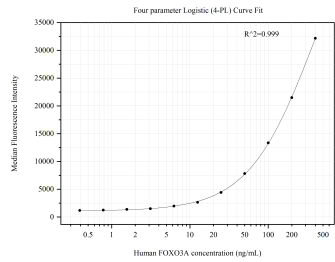
Cytometric bead array standard curve of MP51341-1, FOXO3A Monoclonal Matched Antibody Pair, PBS Only. Capture antibody: 66428-1-PBS. Detection antibody: 66428-2-PBS. Standard:Ag1289. Range: 0.391-400 ng/mL
