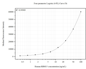
Cytometric bead array standard curve of MP51442-1, RBM15 Monoclonal Matched Antibody Pair, PBS Only. Capture antibody: 66059-1-PBS. Detection antibody: 66059-2-PBS. Standard: Ag17970. Range: 0.391-100 ng/mL.
