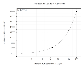
Cytometric bead array standard curve of MP51804-1, EIF3H Monoclonal Matched Antibody Pair, PBS Only. Capture antibody: 61110-1-PBS. Detection antibody: 61110-2-PBS. Standard: Ag30831. Range: 0.781-100 ng/mL.
