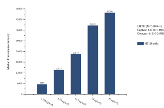
Cytometric bead array sample test of MP51804-1, EIF3H Monoclonal Matched Antibody Pair, PBS Only. Capture antibody: 61110-1-PBS. Detection antibody: 61110-2-PBS.
