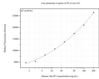
Cytometric bead array standard curve of MP51634-1, AKAP7 Monoclonal Matched Antibody Pair, PBS Only. Capture antibody: 61062-1-PBS. Detection antibody: 61062-2-PBS. Standard: Ag28790. Range: 1.563-200 ng/mL.
