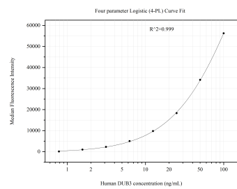
Cytometric bead array standard curve of MP51261-1, DUB3 Monoclonal Matched Antibody Pair, PBS Only. Capture antibody: 60851-1-PBS. Detection antibody: 60851-2-PBS. Standard:Ag24012. Range: 0.781-100 ng/mL
