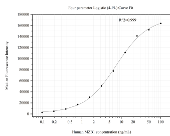
Cytometric bead array standard curve of MP50905-1, MZB1 Monoclonal Matched Antibody Pair, PBS Only. Capture antibody: 60633-1-PBS. Detection antibody: 60633-2-PBS. Standard:Ag17912. Range: 0.098-100 ng/mL
