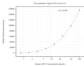
Cytometric bead array standard curve of MP50823-1, ADCY3 Monoclonal Matched Antibody Pair, PBS Only. Capture antibody: 60581-1-PBS. Detection antibody: 60581-2-PBS. Standard:Ag25859. Range: 0.781-100 ng/mL
