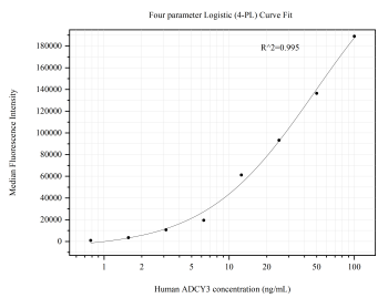
Cytometric bead array standard curve of MP50823-2, ADCY3 Monoclonal Matched Antibody Pair, PBS Only. Capture antibody: 60581-3-PBS. Detection antibody: 60581-2-PBS. Standard:Ag25859. Range: 0.781-100 ng/mL
