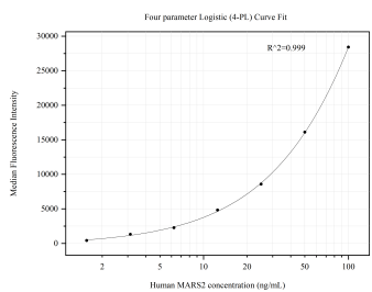
Cytometric bead array standard curve of MP50670-2, MARS2 Monoclonal Matched Antibody Pair, PBS Only. Capture antibody: 60484-3-PBS. Detection antibody: 60484-1-PBS. Standard:Ag18596. Range: 1.563-100 ng/mL.
