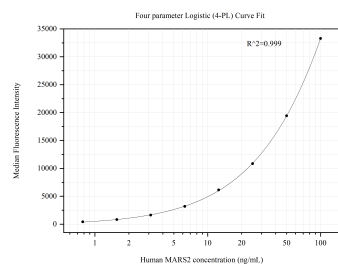
Cytometric bead array standard curve of MP50670-1, MARS2 Monoclonal Matched Antibody Pair, PBS Only. Capture antibody: 60484-1-PBS. Detection antibody: 60484-2-PBS. Standard:Ag18596. Range: 0.781-100 ng/mL.
