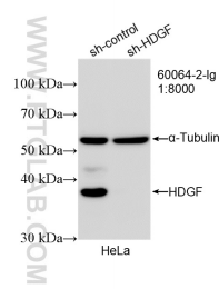
WB result of HDGF antibody (60064-2-Ig; 1:8000; incubated at room temperature for 1.5 hours) with sh-Control and sh-HDGF transfected HeLa cells.
