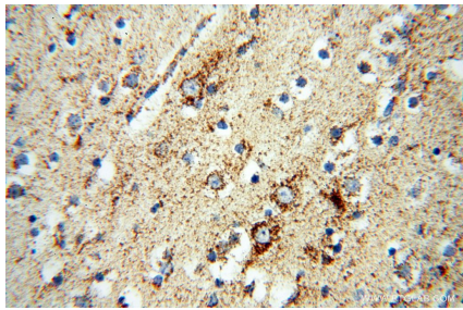
Immunohistochemical analysis of paraffin-embedded human brain using 14912-1-AP (NDUFB7 antibody) at dilution of 1:100 (under 40x lens).
