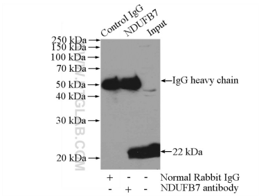
IP result of anti-NDUFB7 (IP:14912-1-AP, 3ug; Detection:14912-1-AP 1:500) with mouse brain tissue lysate 2640ug.
