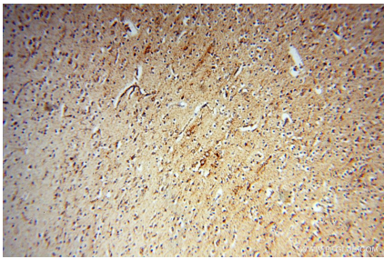
Immunohistochemical analysis of paraffin-embedded human brain using 14912-1-AP (NDUFB7 antibody) at dilution of 1:100 (under 10x lens).
